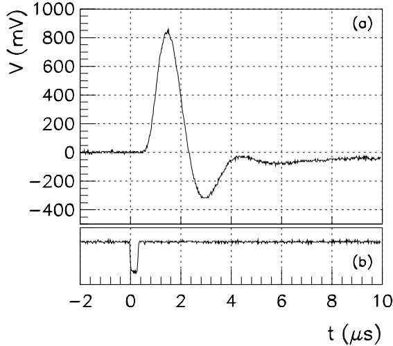
Figure 3. (a) Typical solar cell response with an ORTEC 142B preamplifier to a \Delta t = 300 \text{ ns} light flash; (b) square pulse driving the LED emission.
