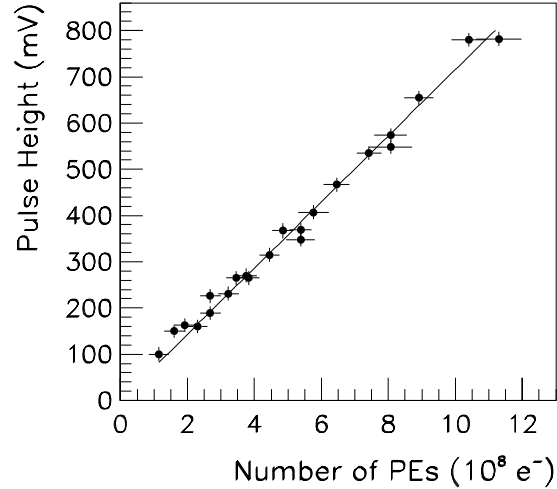
Figure 4. Pulse height versus number of photoelectrons for a 78 \text{ cm}^2 solar cell. The amplifier used is the ORTEC 142B.
