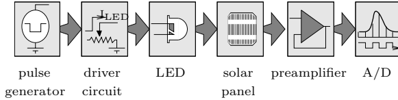
Figure 2. Block diagram of the experimental setup used to evaluate the response of solar cells/panels to light pulses.
