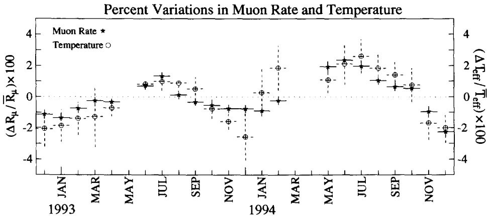
Fig. 4. The superposition of the mean monthly variations in the muon rate, \Delta R_{\mu} / \bar{R}_{\mu} (\%) , and the mean monthly variations in the effective temperature, \Delta T_{eff} / \bar{T}_{eff} (\%) for the December 1992–1994 data set.
