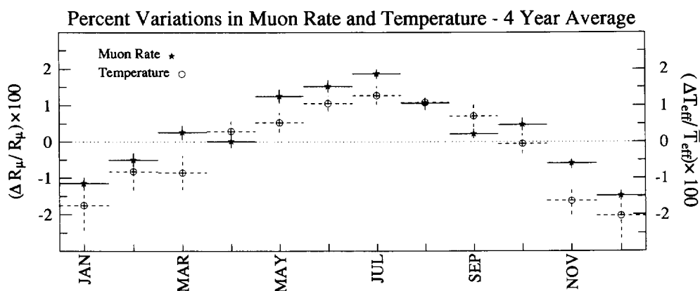
Fig. 5. The superposition of the mean monthly variations in the muon rate, \Delta R_\mu/\bar{R}_\mu (%), and the mean monthly variations in the effective temperature, \Delta T_{eff}/\bar{T}_{eff} (%) for the averaged total data set, 1991–1994.
