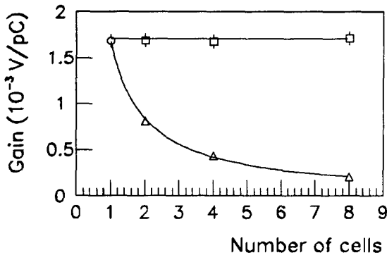
Figure 5. Voltage-to-charge gain for different electrical connections of identical cells. □: series connection; △: parallel connection.
