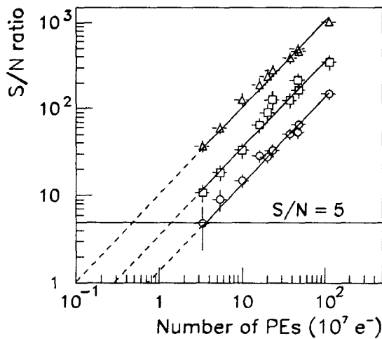
Figure 7. Signal-to-noise ratio versus the number of PEs for three different solar panels. ○: 36 \cdot 96 \text{ cm}^2 mono-Si cells; □: 32 \cdot 32 \text{ cm}^2 a-Si cells; △: 36 \cdot 9 \text{ cm}^2 mono-Si cells.
