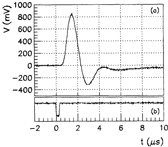
Figure 3. (a) Typical solar cell response with an ORTEC 142B preamplifier to a \Delta t = 300 ns light flash; (b) square pulse driving the LED emission.
