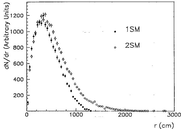
FIG. 4. Muon separation distributions measured by MACRO with one supermodule (144 m 2 horizontal area) and two supermodules (288 m 2 horizontal area).
