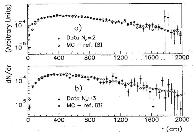
FIG. 10. Comparison of the experimental decoherence distribution for (a) the dimuon sample and (b) the trimuon sample with the simulation performed using the parametrization of Ref. [8].
