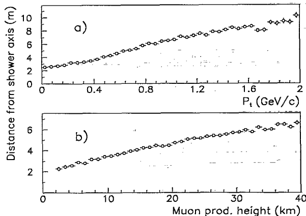
FIG. 12. Average distance from the shower axis for muon bundles detected underground (a) vs the transverse momentum of parent mesons and (b) vs the muon production height measured along the shower axis.
