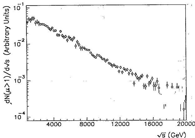
FIG. 3. Distribution of the muon bundles ( n_{\mu} \geq 2 ) as function of the nucleus-nucleus center-of-mass energy ( \sqrt{s} ) of the primary interaction, as given by the HEMAS code using the CMC model.
