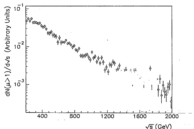
FIG. 1. Distribution of the muon bundles ( n_\mu \geq 2 ) vs the nucleon-nucleon center-of-mass energy ( \sqrt{s} ) of the primary interactions, as given by the HEMAS code using the CMC model.
