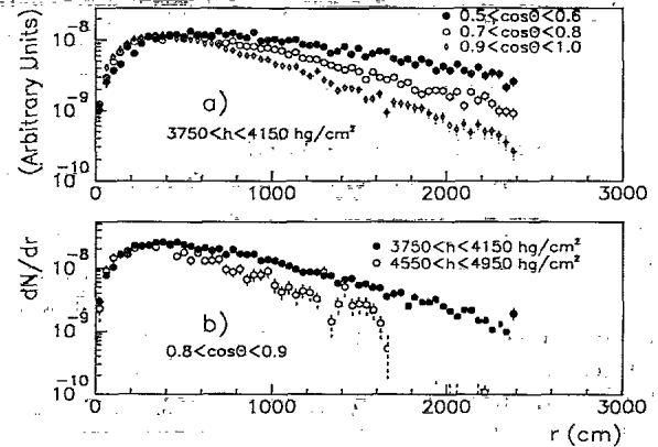
FIG. 13. Simulated decoherence function in a fixed rock depth interval (a) for three different zenith ranges and (b) in a fixed zenith-angle interval for two different ranges of rock depth.
