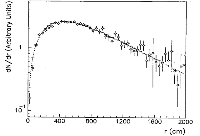
FIG. 6. Comparison of the input distance distribution and the reconstructed function using the second unfolding method (see Sec. V B). Dotted line, input function; points with error bars, results of the unfolding procedure.
