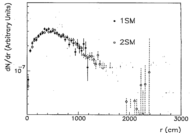
FIG. 7. Comparison of the decoherence functions for one (solid circles) and two (open circles) supermodules.
