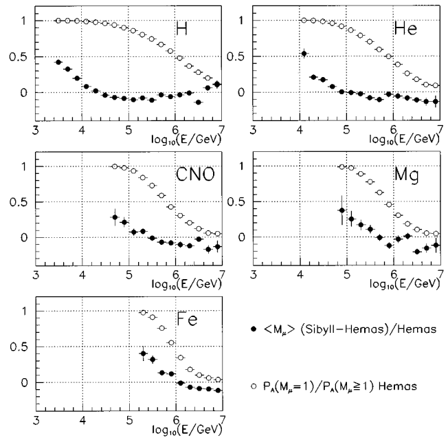
FIG. 2. Full circles: relative differences between SIBYLL and HEMAS average muon multiplicities at MACRO: (S-H)/H. Open circles: fraction of single muons as with HEMAS code.
