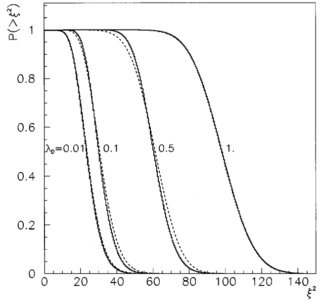
FIG. 16. Cumulative probability distributions P(\geq \xi^2) [Eq. (B2), in the text] for different values of \lambda_D (solid histograms). For comparison, dashed lines show the cumulative \chi^2 probabilities for \lambda_M \nu_M + \lambda_D \nu_D degrees of freedom.
