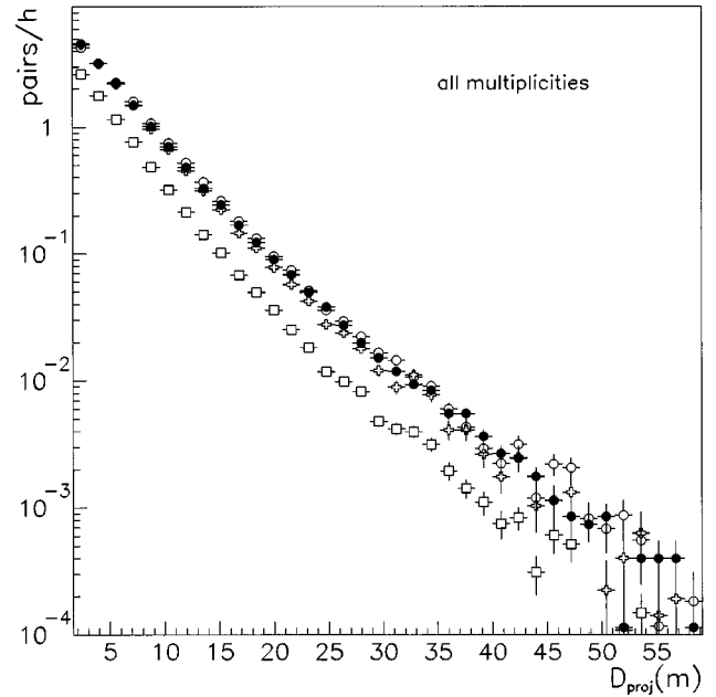
FIG. 14. Comparison between experimental and predicted muon lateral separations, in MACRO, projected in the wire view for events with any multiplicity. Same symbols as in Fig. 13. Projected separations lower than 1 m have not been considered because of experimental inefficiencies in the close track separation. Here each muon pair enters with unit weight.
